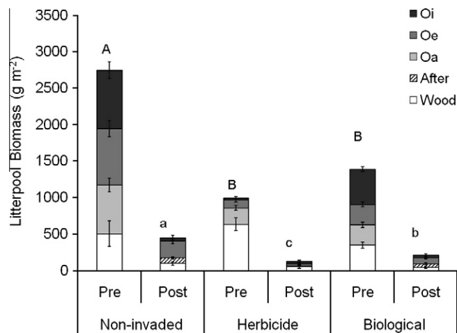
Fig. 1. Mean ( \pm SE) of pre- and post-fire biomass of all litter components (Oi, Oe, Oa, after, and wood) measured in the non-invaded, herbicide, and biological control sites (Different capital and lower case letters indicate significant differences for pre- and post-fire means, respectively).
