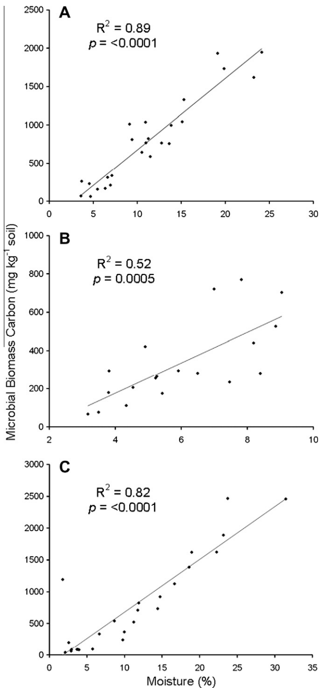
Fig. 3. Relationship between microbial biomass carbon concentration and percent soil moisture in the pre-fire, 0–5 cm soil depth of the (A) non-invaded, (B) herbicide, and (C) biological control sites.
