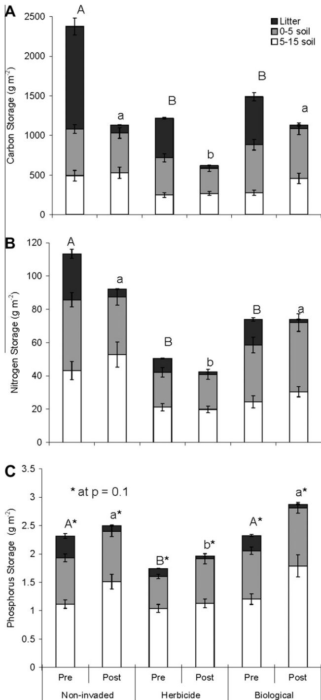
Fig. 2. Mean ( \pm SE) of pre- and post-fire total storages of (A) carbon, (B) nitrogen, and (C) phosphorus measured in the non-invaded, herbicide, and biological control sites (Different capital and lower case letters indicate significant differences for pre- and post-fire means, respectively).
